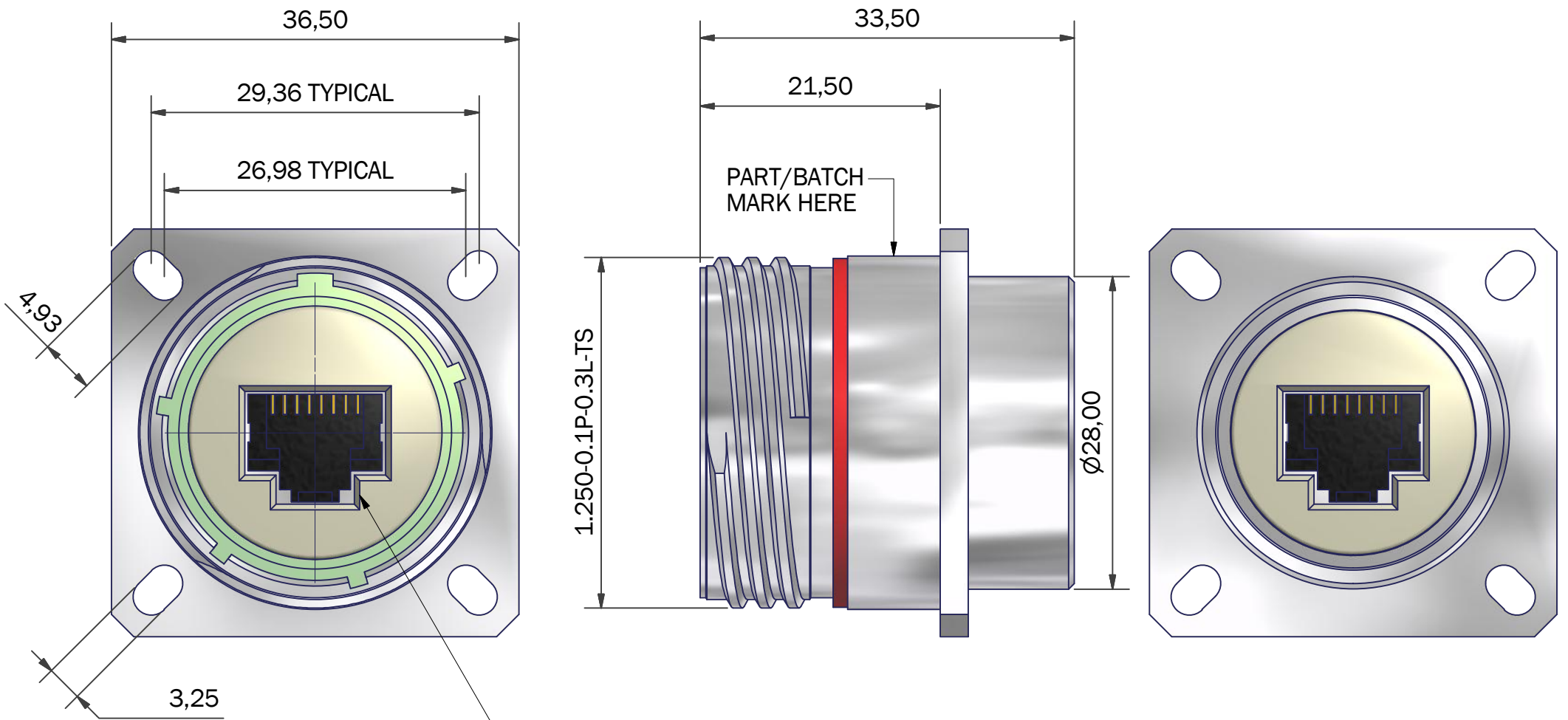
RJ45, CAT6a (10Gb) FEEDTHROUGH CONNECTOR GROUNDED TO OUTER SHELL
